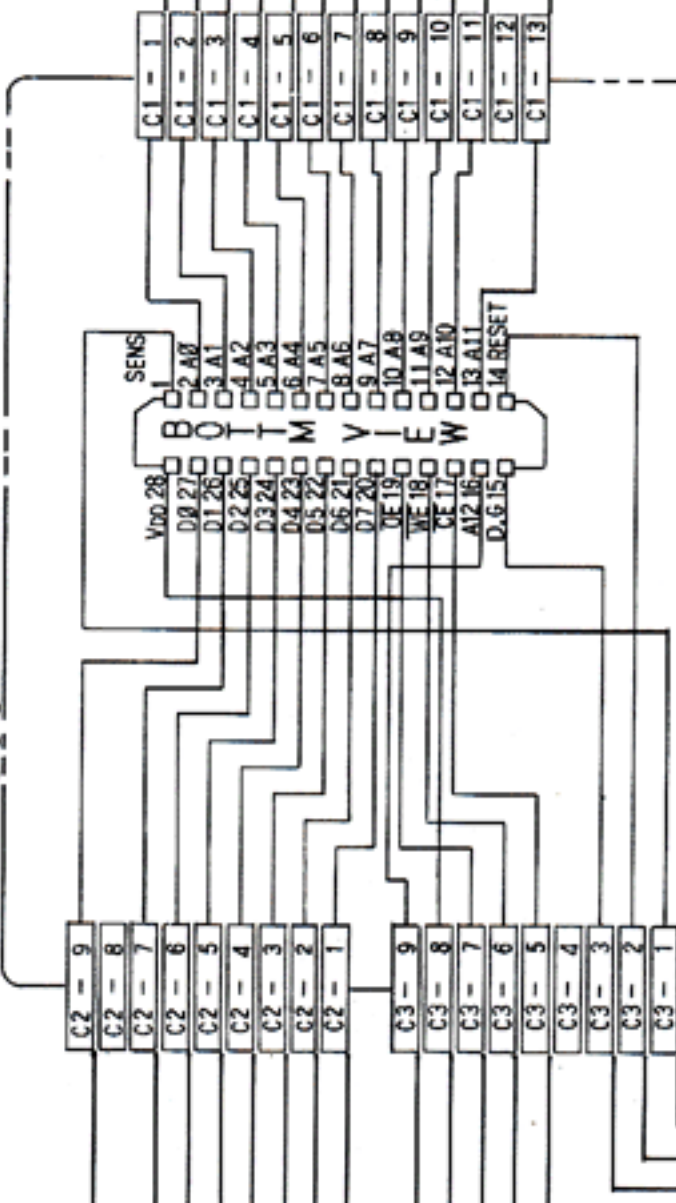
CARTRIDGE BOARD 793406000
