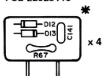
ATTACK BOARD PCB 22925119
