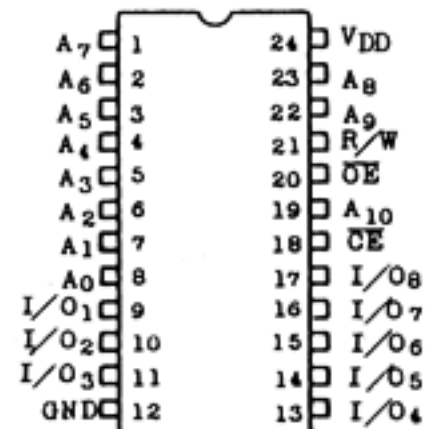
Pin Configuration
