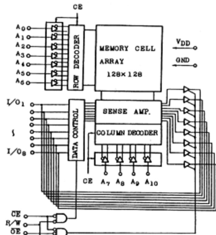
Block Diagram
