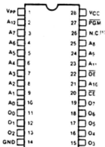
Pin Configuration
