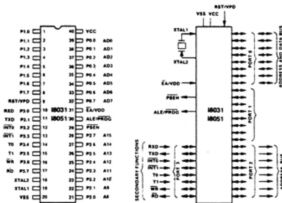
Pin Configuration
