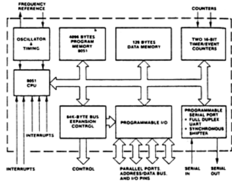
Block Diagram
