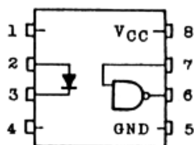
Pin Configuration
