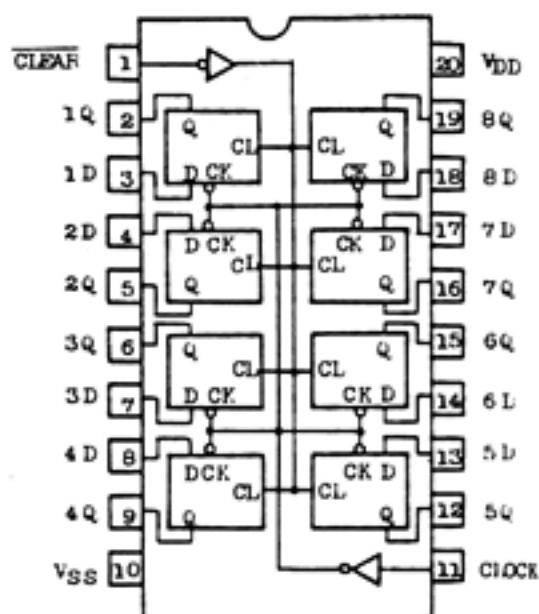
Pin Configuration
