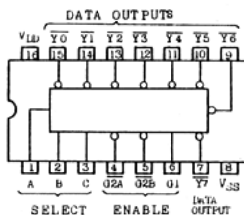
Pin Configuration
