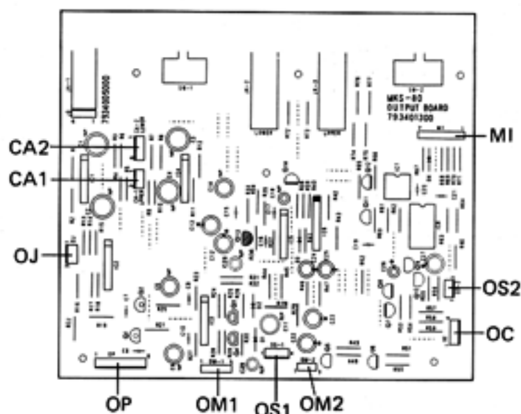
OUTPUT BOARD
