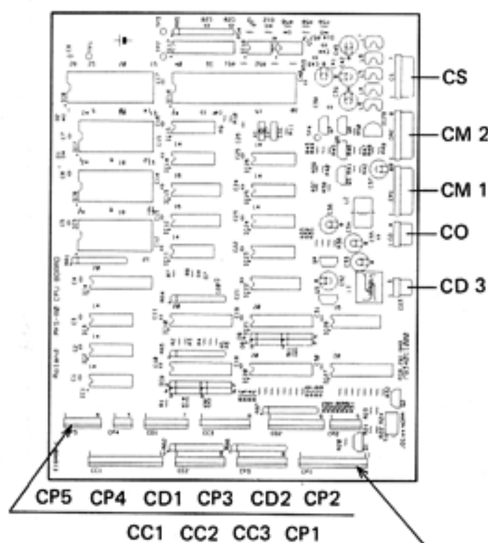
CPU BOARD
