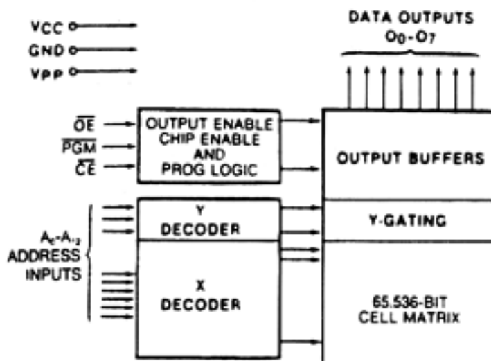
Block Diagram
