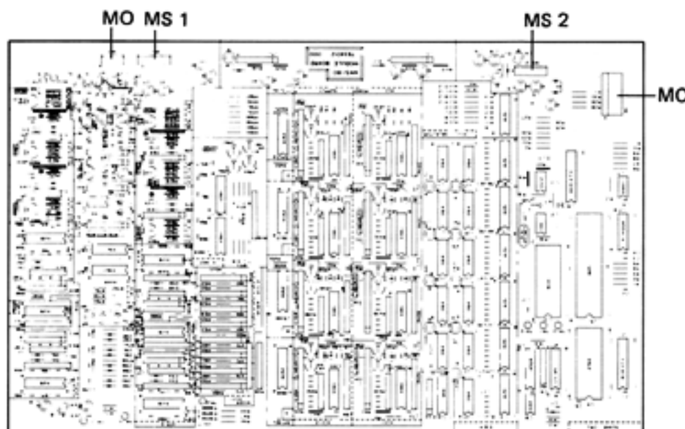
MODULE BOARD
