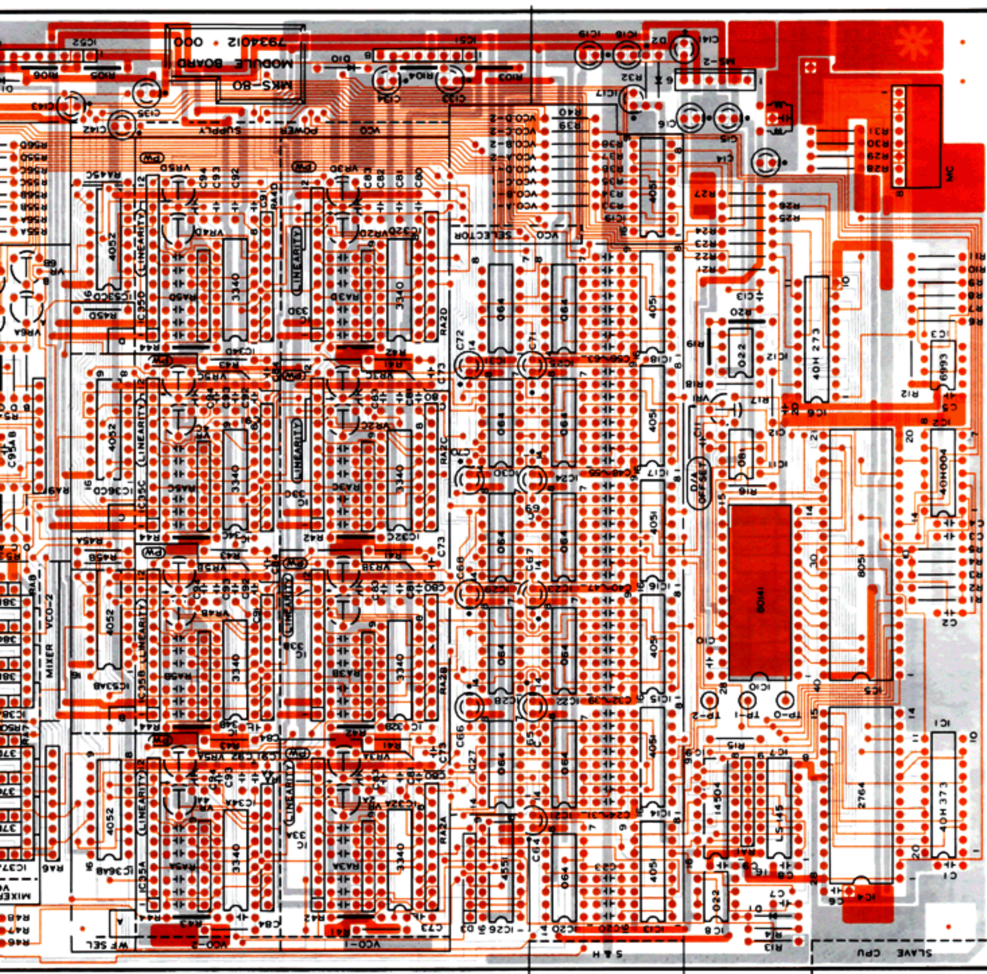
A, B, C, D; MODULE BOARD 4 Voice
